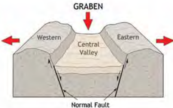
Fig. 6 Connecticut's Central Valley may have started to form as a graben but more rapid downward motion along eastern faults soon initiated eastward tilting of the valley's down-dropping metamorphic blocks.
