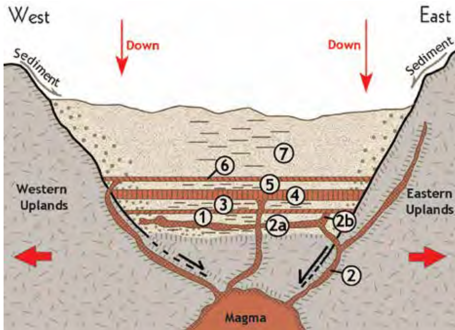
Fig. 7 Idealized cross-section of the Central Valley showing the relationship of its geologic components (not to scale) as they were emplaced during tilting (note different magnitude of red “Down” arrows). At this stage in the development of the valley successive sedimentary deposits and intervening lava flows formed alternating layers above the eastward tilting metamorphic blocks. The sedimentary and igneous rock units depicted are, from oldest to youngest: 1) New Haven Arkose; dikes feeding the diabase sills (2a) that intruded the New Haven Arkose and fed the lava (2b) that formed the Talcott Basalt; 3) Shuttle Meadow Formation; 4) Holyoke Basalt; 5) East Berlin Formation; 6) Hampton Basalt; 7) Portland Arkose.
